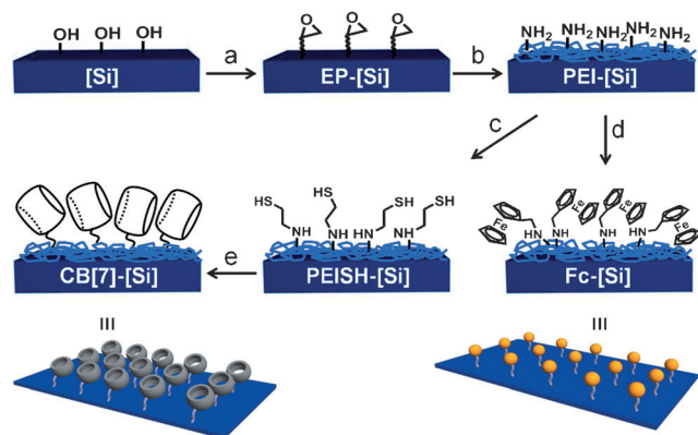
Figure 2. Preparation of CB[7]- and Fc-functionalized silicon surfaces. a) Incubation of hydroxy terminated [Si] in 3-glycidoxypolytrimethoxysilane (3-GPTS) solution to give epoxy termini in EP-[Si]. b) Epoxide ring opening with branched-polyethyleneimine to give amine functionalized PEI-[Si]. c) Reaction with ethylene sulfide resulting in thiol-functionalized PEISH-[Si]. d) Anchoring of Fc groups by condensation with ferrocenecarboxaldehyde followed by reduction with \text{NaBH}_4 , resulting in Fc-[Si]. e) Thiol-ene “click” reaction between (allyloxy) 1 CB[7] and PEISH-[Si] to give CB[7]-[Si]. Note that the schematic drawings of CB[7]-[Si] and Fc-[Si] are highly simplified and the actual structures of the PEI layers, wherein CB[7] and Fc anchored, are highly complex.
